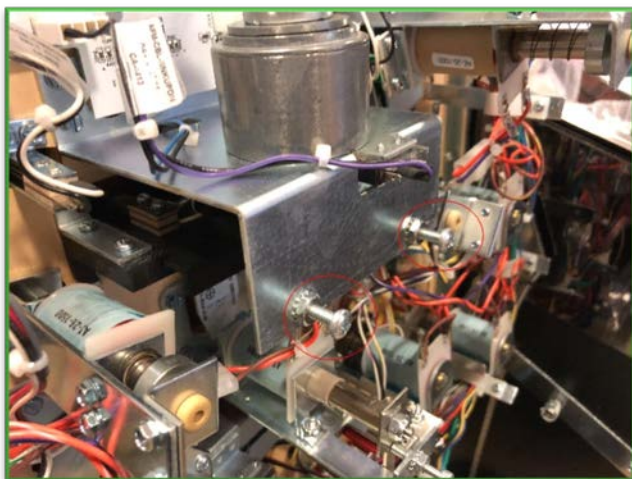
Adjusting screws
